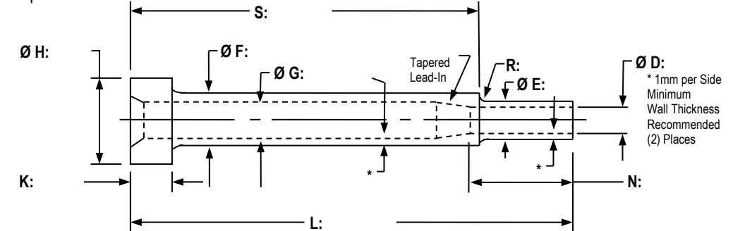
Step Sleeve
