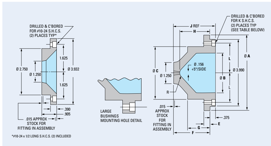
Runner Stripper Plate Bushing TEB-0001
