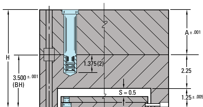
SECTION Z-Z REF.
