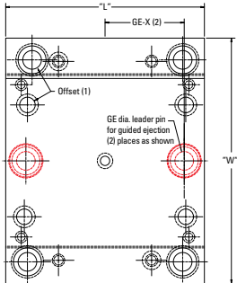
"B" HALF OF MOLD FOR 88 & 812 MOLD BASES ONLY
