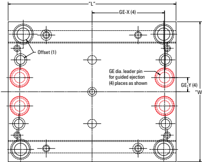
"B" HALF OF MOLD FOR 108 - 2435 BASES
