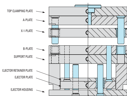
AX-Series Assembly
