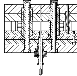
SECTION B-B EJECTOR PLATES BACK - MOLD OPEN
