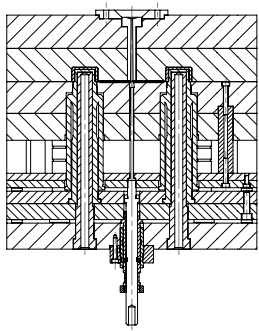
SECTION A-A EJECTOR PLATES BACK - MOLD CLOSED
