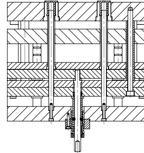
SECTION C-C FIRST EJECTOR STROKE
