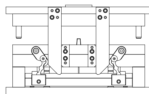
MOLD CONTINUES CLOSING
