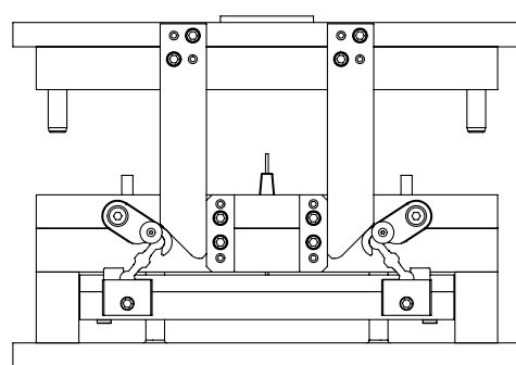
MOLD CLOSING
