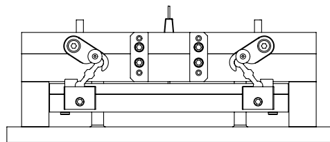
MOLD FULL OPEN
