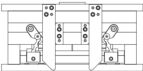
MOLD CLOSED IN MOLDING POSITION
