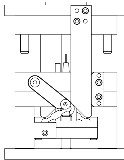
MOLD CLOSING
