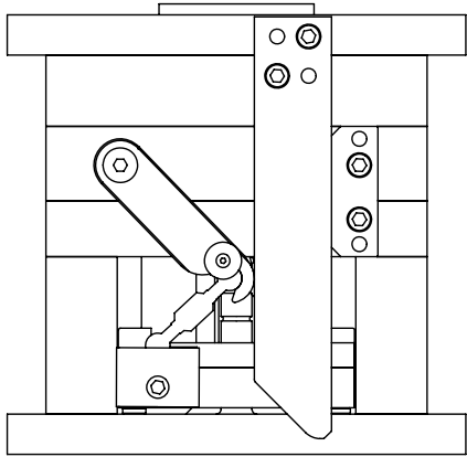
MOLD CLOSED IN MOLDING POSITION
