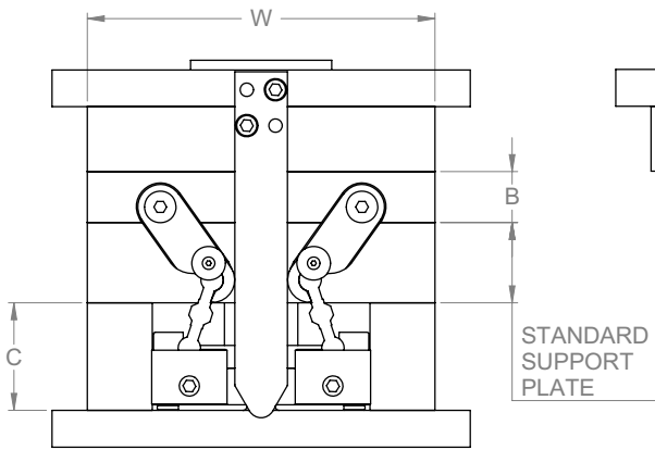
MOLD CLOSED IN MOLDING POSITION
