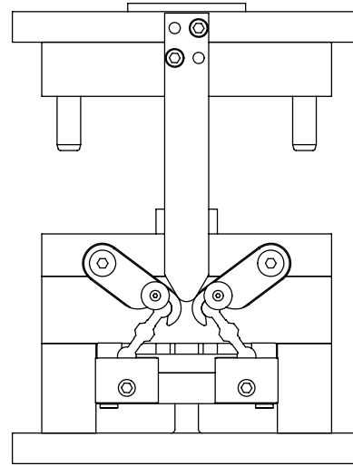
MOLD CLOSING
