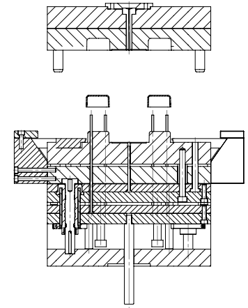
SECTION E-E
