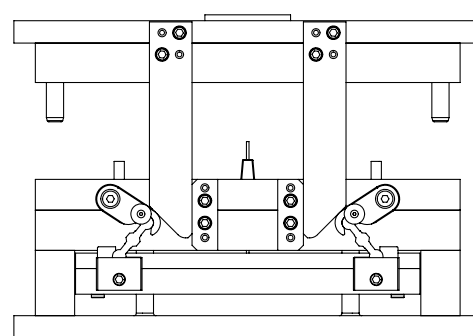
MOLD CLOSING
