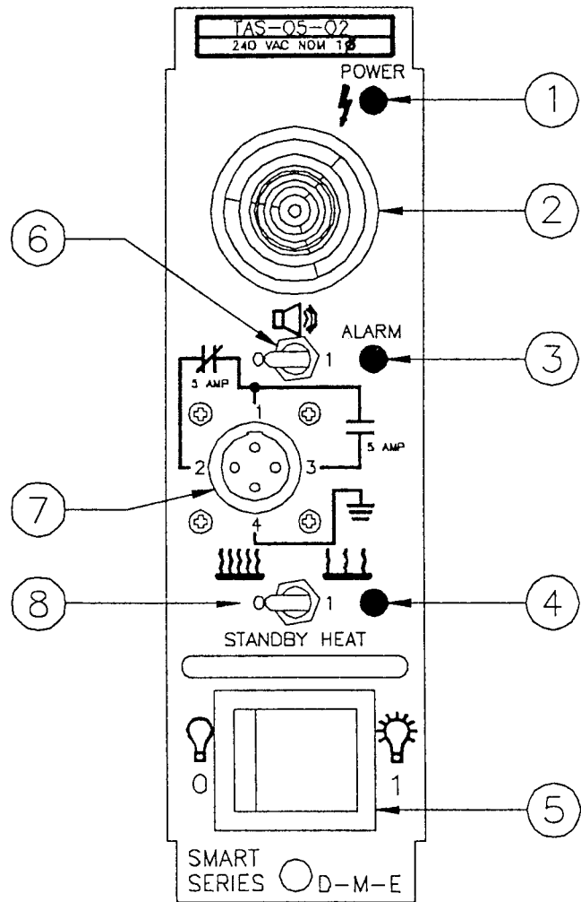
Figure 1. - TAS-05-02 Module
