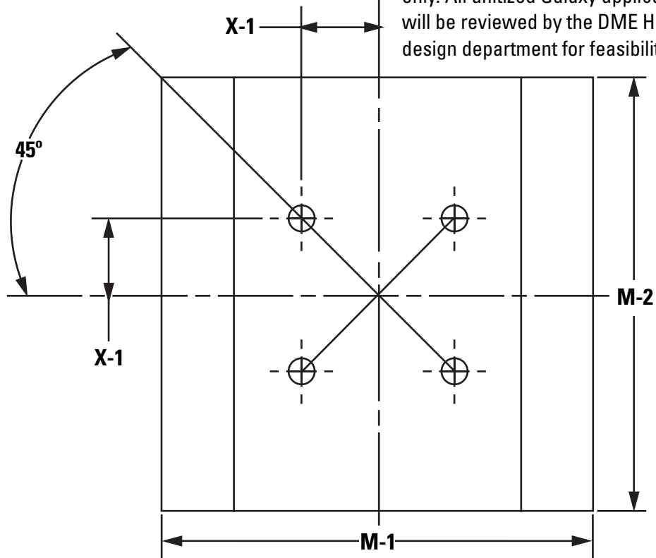
MINIMUM MOLD BASE SIZE
