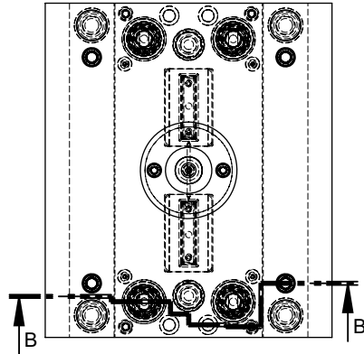
EARLY EJECTOR RETURN ASSEMBLY - ACTUATION SEQUENCE
