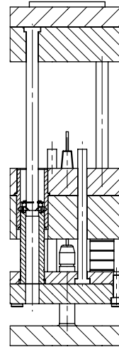
SECTION C-C
