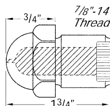
FD-type filter disk in machined recess in rear of regular tip
