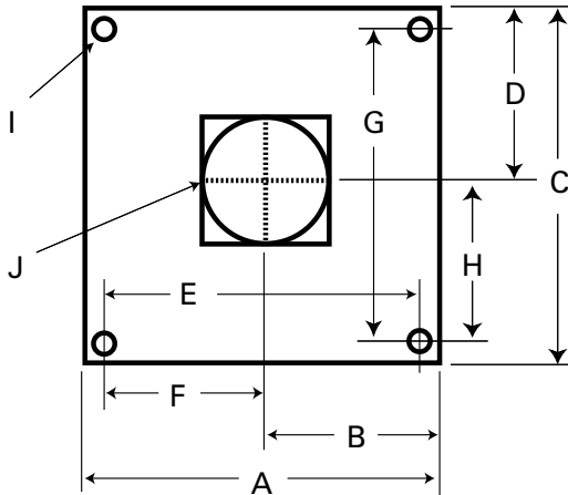
BOTTOM FLANGE OPERATOR SIDE (FRONT)
