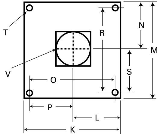
TOP FLANGE OPERATOR SIDE (FRONT)
