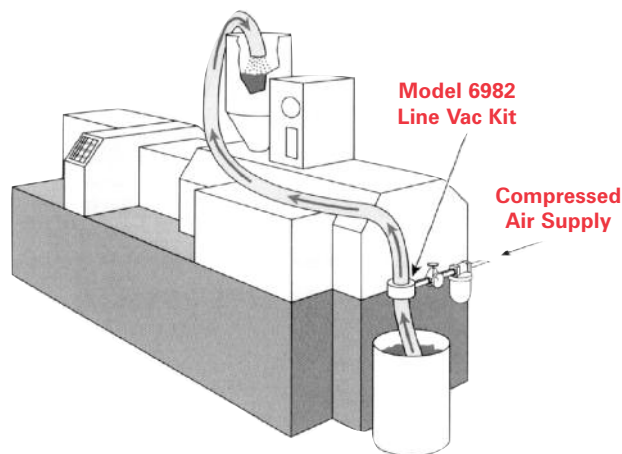
Line Vac Kit includes a Line Vac, mounting bracket, filter separator and a pressure regulator.
