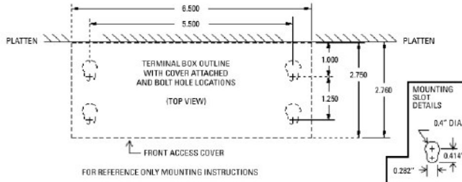
IMB1200 Mounting Box Dimensions – Leave Room for Cover Removal and Access.
